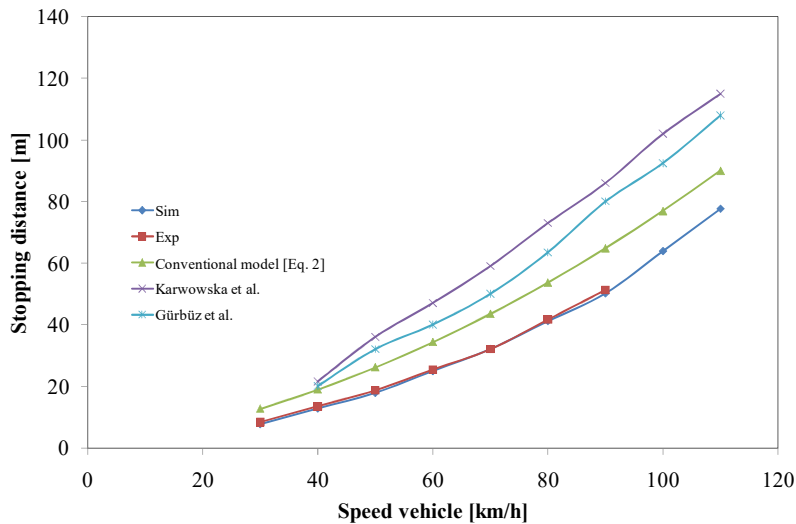
Fig. 6- Comparison of stopping distances.
